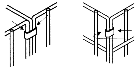
CLIP ATTACHMENT
